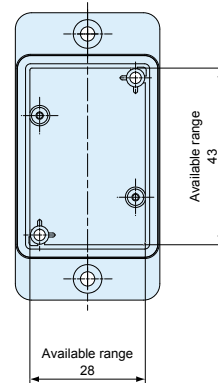
Flanged base (Internal)
