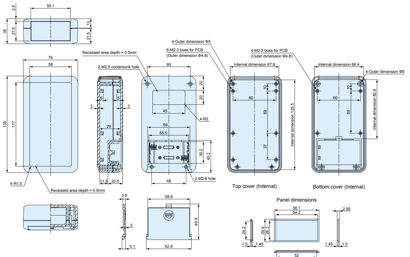
LCT135H-M2 / LCS135H-M2 / LC135H-M2
