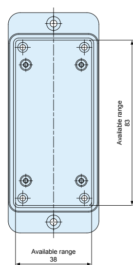
Flanged base (Internal)
