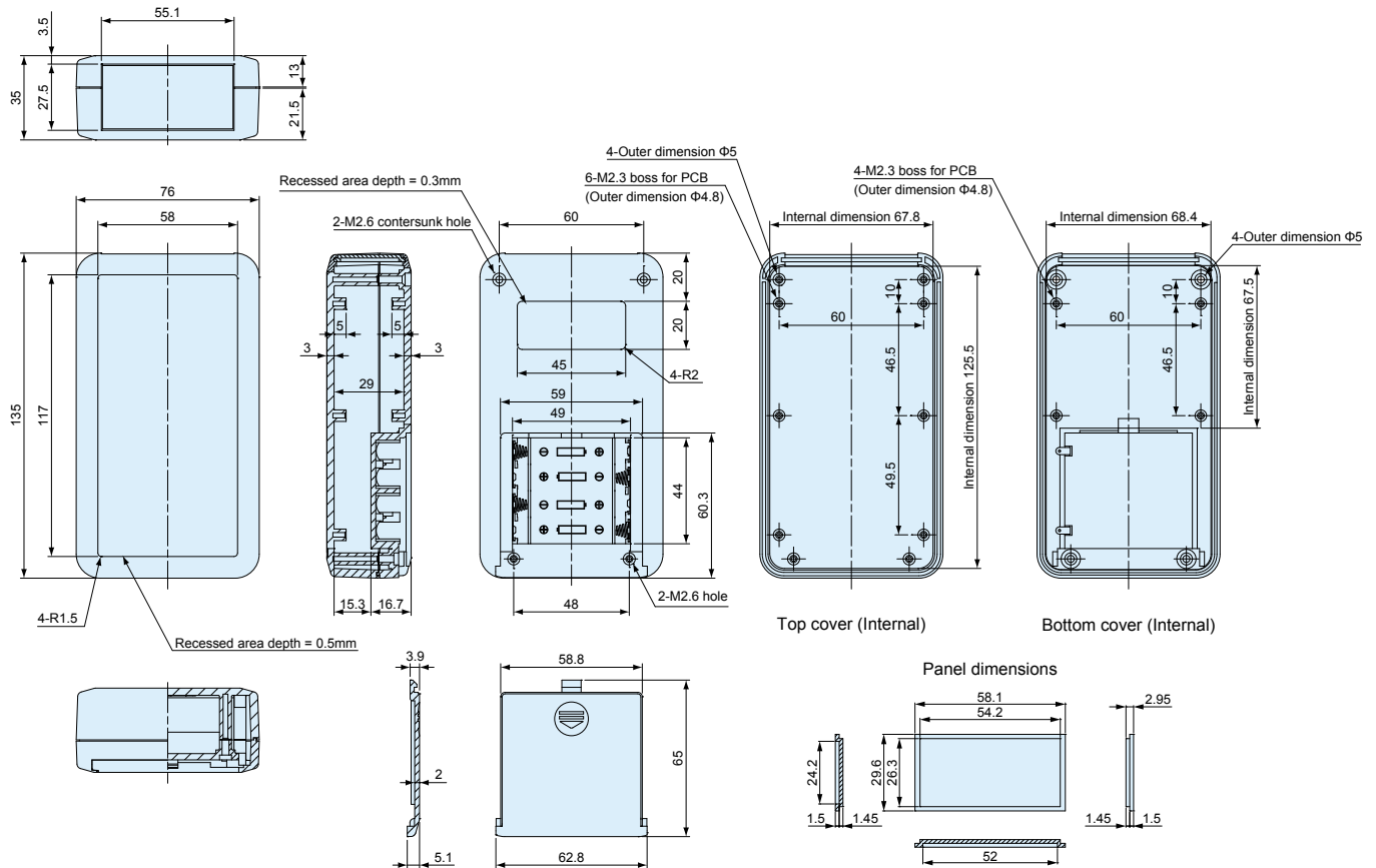
LCT135H-F4 / LCS135H-F4 / LC135H-F4
