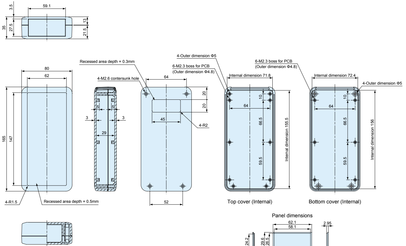
LCT165H-M4 / LCS165H-M4 / LC165H-M4
