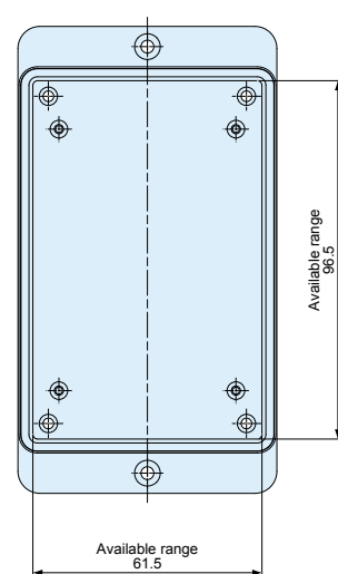
Flanged base (Internal)
