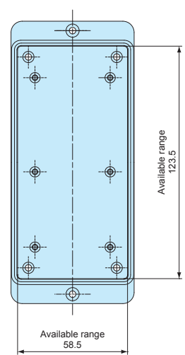
Flanged base (Internal)
