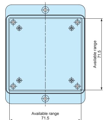
Flanged base (Internal)
