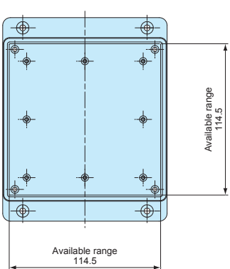
Flanged base (Internal)
