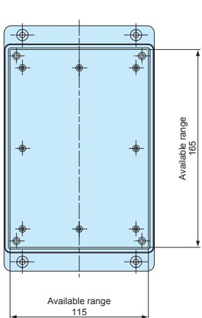
Flanged base (Internal)
