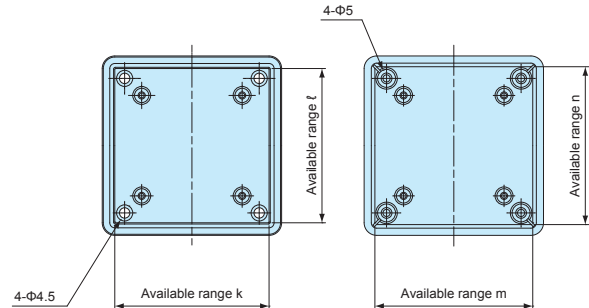
Top cover (Internal)
