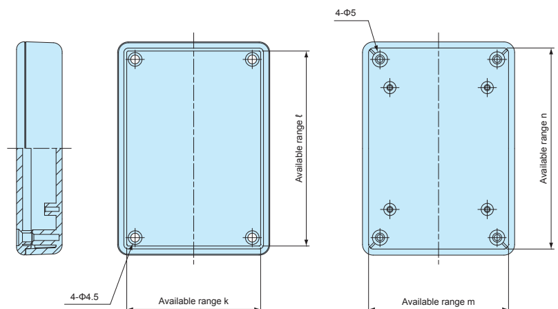
Top cover (Internal)
