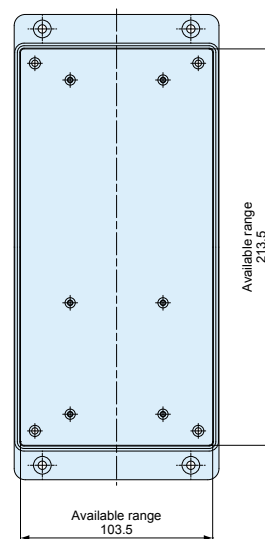
Flanged base (Internal)
