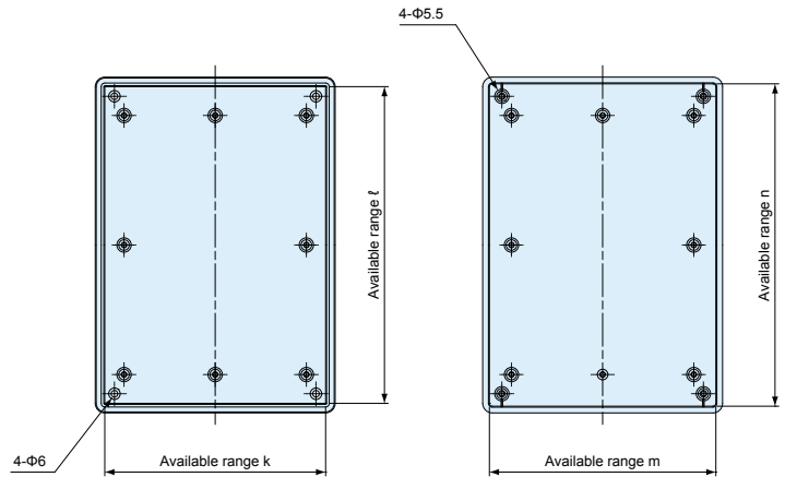
Top cover (Internal)
