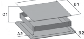
Wandgehäuse Form 2 Wall mount enclosure form 2
