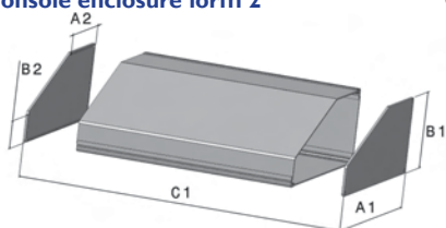
Pultgehäuse Form 2 Console enclosure form 2
