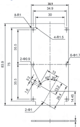
CR2032-Batteriefach CR2032-battery compartment
