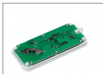
CR2032-Batteriefach CR2032-battery compartment
